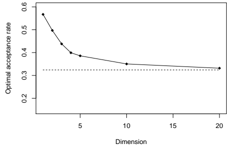
Figure 2: Optimal acceptance rate of the MTM algorithm with K = 2 as a function of the dimension T .
