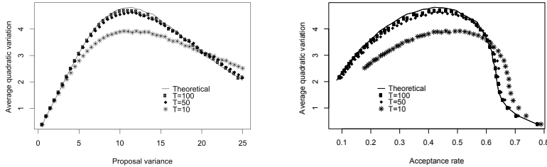
Figure 3: AQV as a function of the proposal variance (left) and the acceptance rate (right) for the MTM algorithm with a normal target and K = 7 independent proposals. The plotted symbols are the results of simulation studies in different dimensions, while the solid lines represent the theoretical curves.
