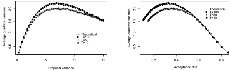
Figure 1: AQV as a function of the proposal variance (left) and the acceptance rate (right) for the MTM algorithm with a normal target and K = 2 independent proposals. The plotted symbols are the results of simulation studies in different dimensions, while the solid lines represent the theoretical curves.
