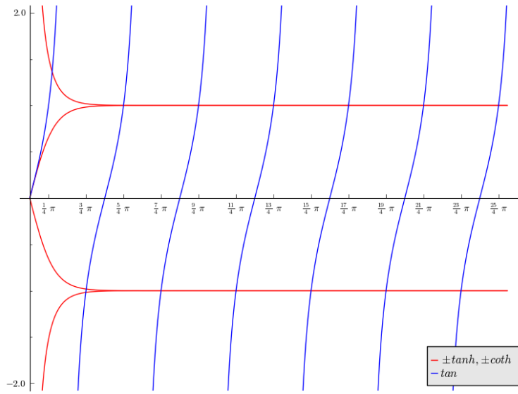
FIGURE 1. The Steklov eigenvalues of a square. Each intersection corresponds to a double eigenvalue.
