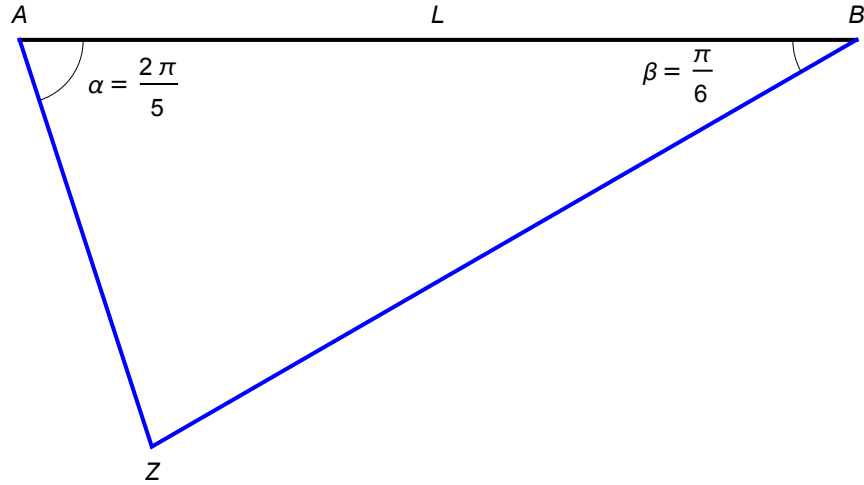
Figure 5: Triangle from Example C.1
